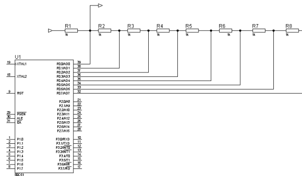
Figure 3. MCU Control Analog to Digital Potentiometer
