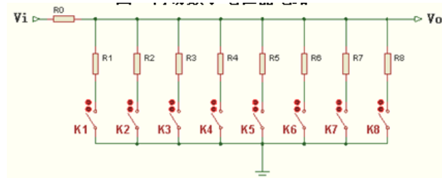
Figure 2. Simple Digital Potentiometer Circuit
