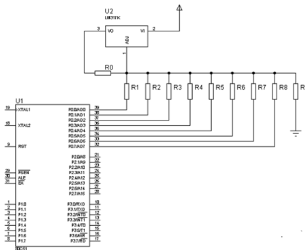
Figure 4. Analog to Digital Potentiometer Constituting the Numerical Control Voltage Source
